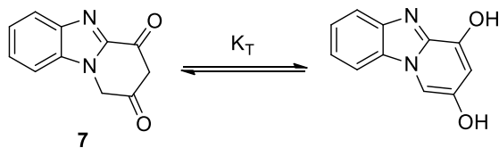
Figure 4: The tautomerism of compound, 7,
